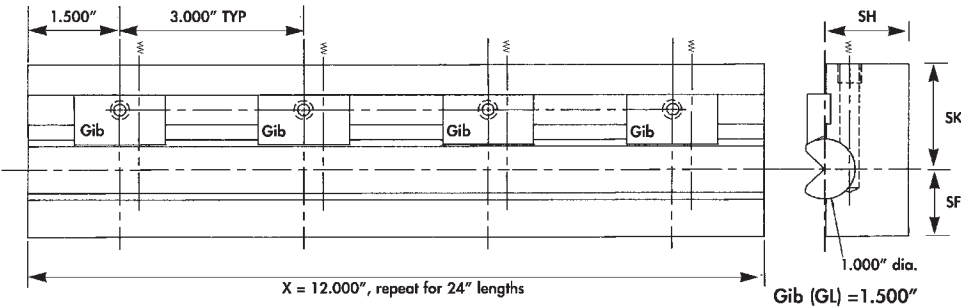
HIB 100: 12" & 24" lengths in stock, 1" Diameter Rocker
