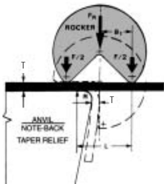
(Clamp position shown solid, overbend position dotted)
