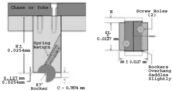
Regular Benders Note: extended rockers (E) are special
